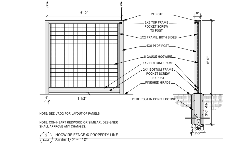
2 HOGWIRE FENCE @ PROPERTY LINE Scale: 1/2" = 1'-0"
