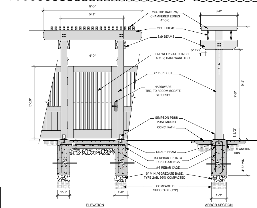
5 WOOD ARBOR & GATE @ WALNUT AVE. Scale: 1/2" = 1'-0"
