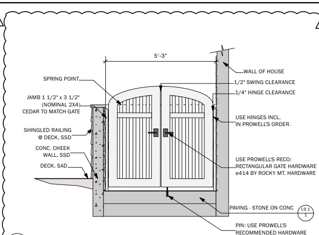
6 GATE @ WEST STEPS - BY PROWELLS Scale: 1/2" = 1'-0"
