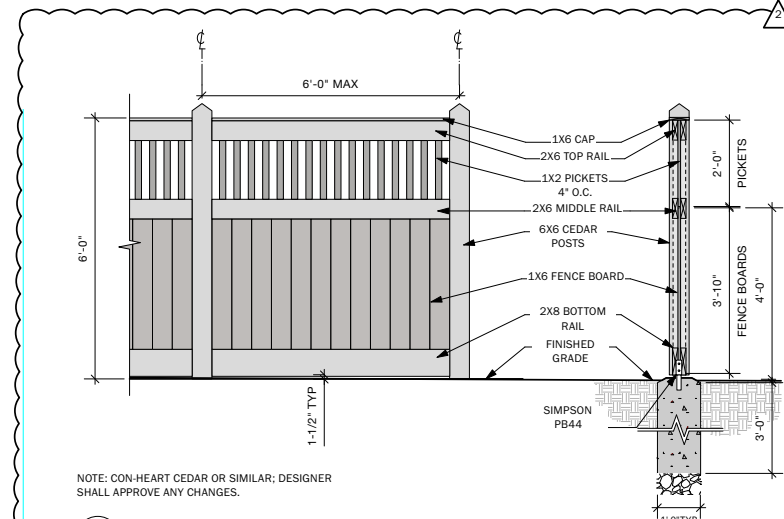
1 FENCE @ WALNUT Scale: 1/2" = 1'-0"
