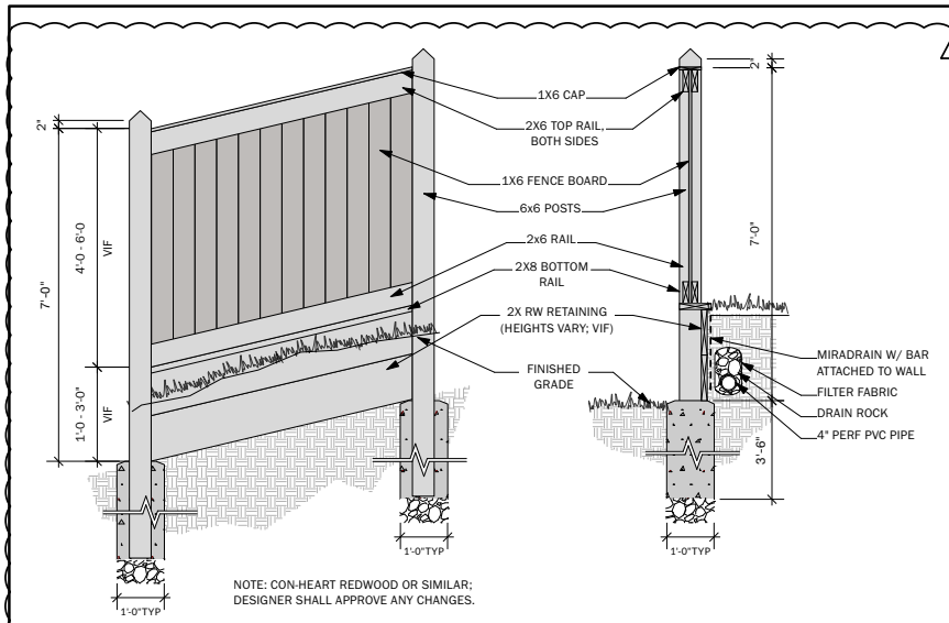
9 7' PRIVACY FENCE @ WEST PROP LINE, NO PICKETS, RETAINING INCLUDED Scale: 1/2" = 1'-0"
