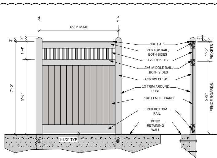
8 7' PRIVACY FENCE WITH PICKETS @ WEST PROP LINE Scale: 1/2" = 1'-0"
