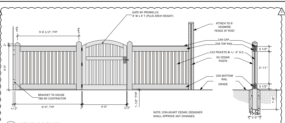
3 4' FENCE @ E. ENTRANCE Scale: 1/2" = 1'-0"
