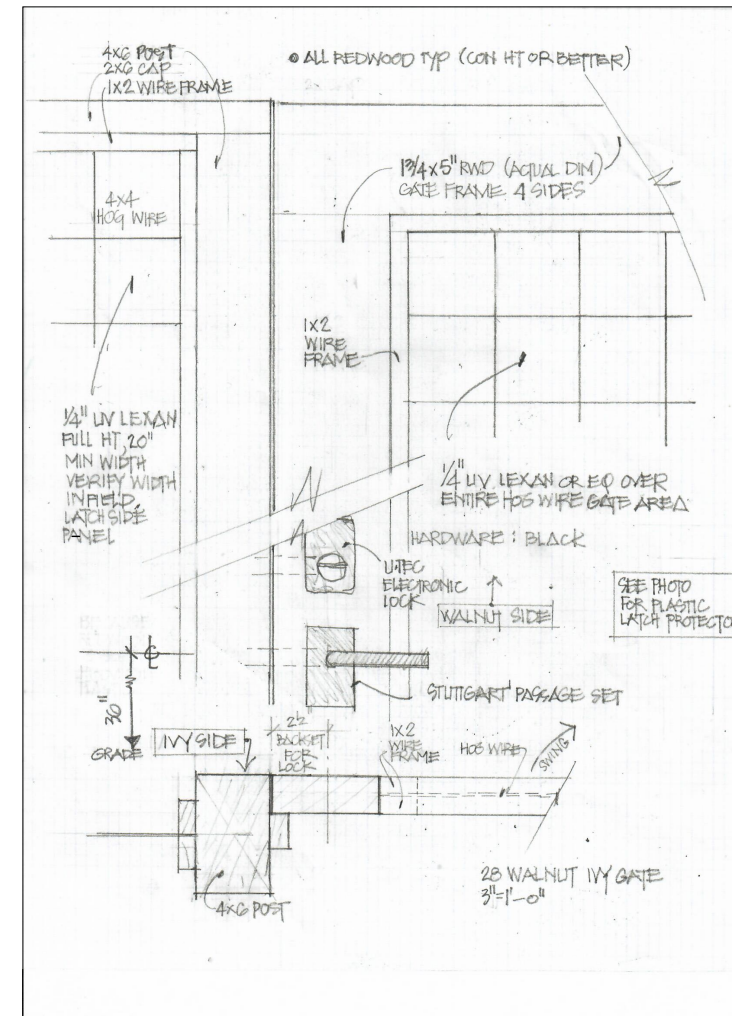
2 IVY GATE HARDWARE Scale: NTS MOVED TO G.C.'S SCOPE
