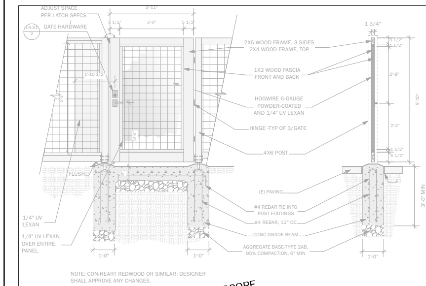
7 GATE - 6' WOOD FRAME W/ HOG WIRE Scale: 1/2" = 1'-0"
