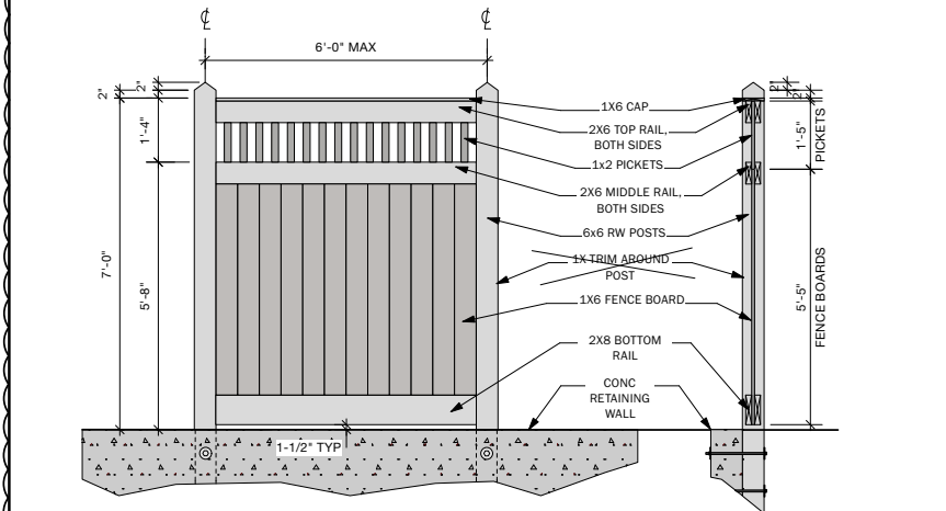
8 7' PRIVACY FENCE WITH PICKETS @ WEST PROP LINE Scale: 1/2" = 1'-0"
