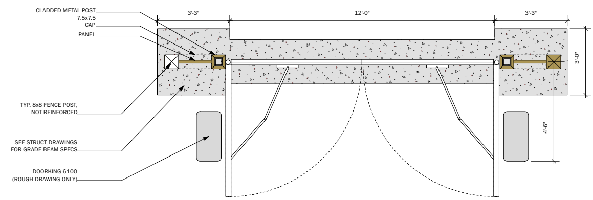
4 PLAN VIEW AUTOGATE, GRADE BEAM, EQUIPMENT Scale: 1/2" = 1'-0"
