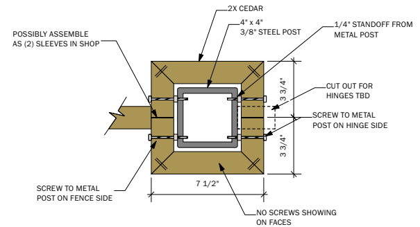
5 WOOD CLADDING ON DRIVEWAY METAL POSTS Scale: 1/2" = 1'-0"
