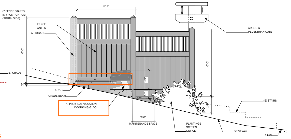
1 EAST FENCE AT AUTOGATE/DRIVE (DOORING EQUIP) Scale: 1/2" = 1'-0"
