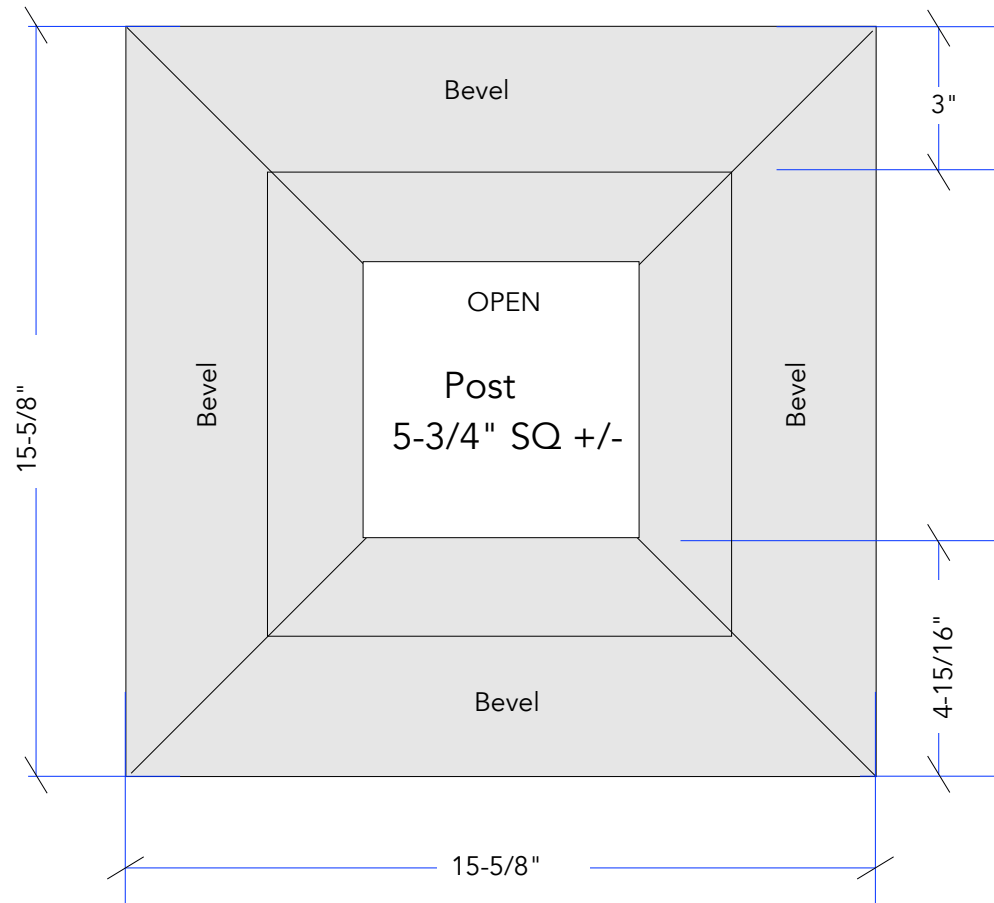
PLAN VIEW OF CAPS
