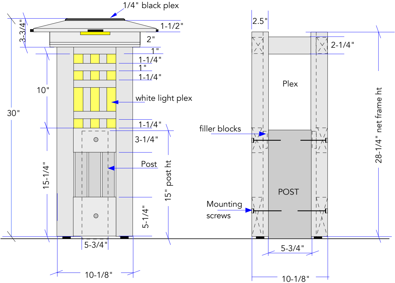
CROSS-SECTION SIDE VIEW
